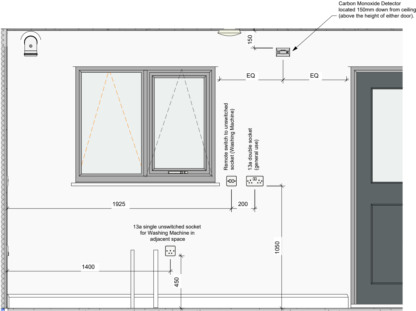
C Kitchen Electrics - View C (Rented Spec) 1 : 20
