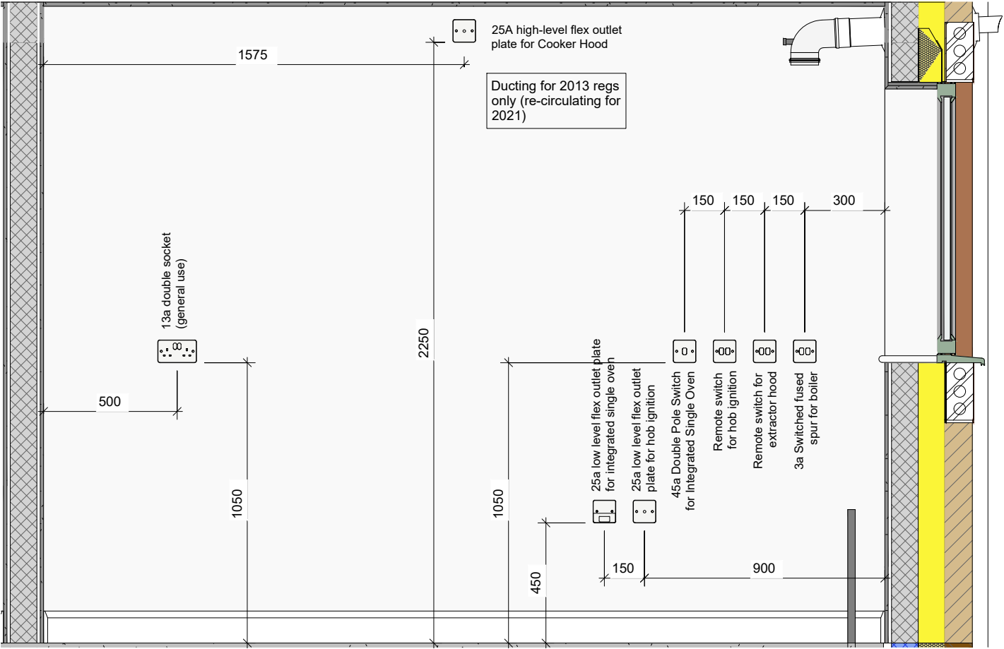
B Kitchen Electrics - View B (Rented Spec) 1 : 20
