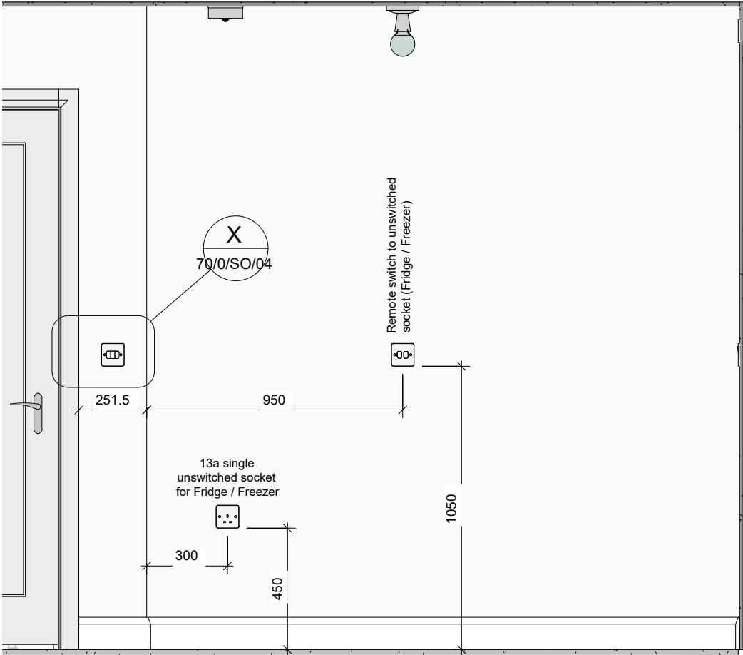
A Kitchen Electrics - View A (Rented Spec) 1 : 20
